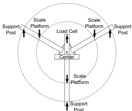
Figure 1. Simplified diagram showing top view of the scale mechanism. The three arms of the mechanism are arranged around a common central point, with the two diagonal arms being able to pivot in the vertical direction. The outer circle shows the positions of support posts, which the arms rest on. The inner circle shows the positions where the scale platform rests on top of the arms. The end of the central arm rests on the load cell. As the load is applied to the scale platform, the arms transmit the force to the load cell which flexes. The equidistant arrangement ensures that each arm tilts the same amount, hence limiting the change of orientation of the SQUID.
