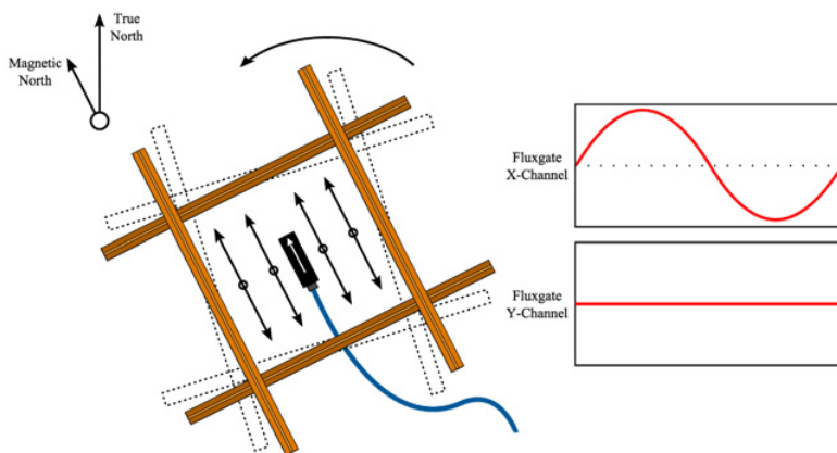
Figure 4. Fluxgate magnetometer used to align coils to Magnetic North.
