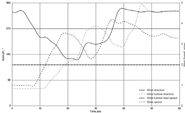
Fig. 4. The registered parameters of wind turbine.
