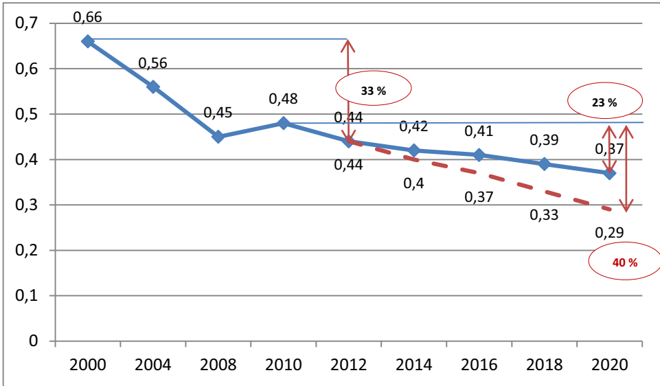
Fig. 1. Energy intensity changing per unit of GDP in Russia from 2000 to 2020, tons of equivalent fuel per $ 1,000.
