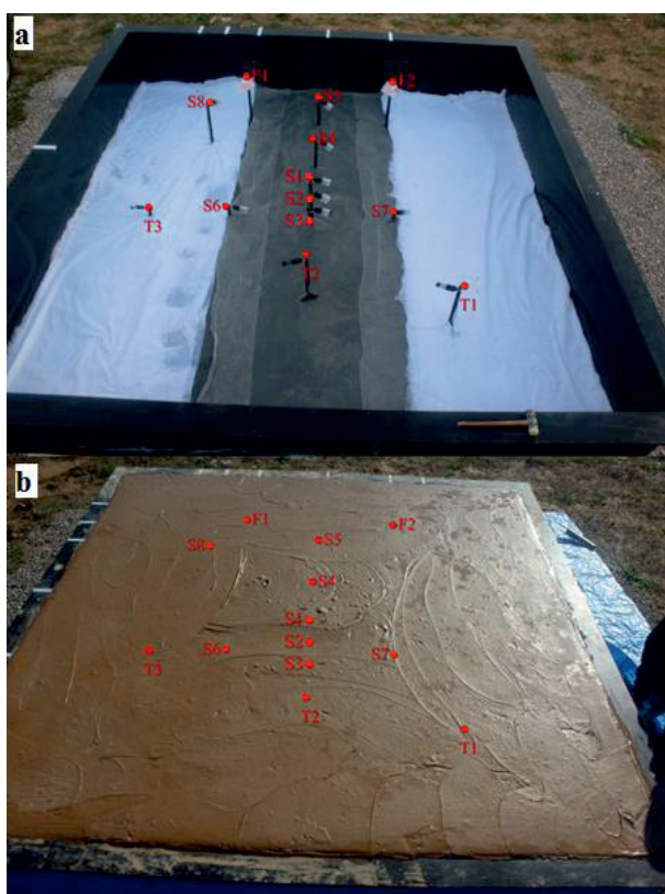
Figure 2. Distribution of the internal sensors. (S1-S8) Suction sensors; (T1-T3) VWC, temperature and EC; (F1-F2) Heat flux. (a) Container, geotextile & indoor sensors. (b) Initiation of the test.
