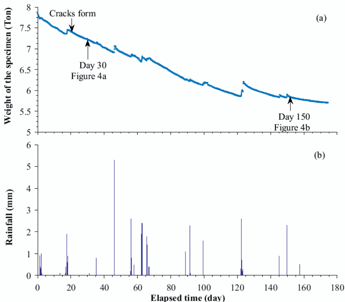
Figure 3. Natural wetting plotted against time. (a) Weight of the specimen evolution. (b) Rainfall by weather station.
