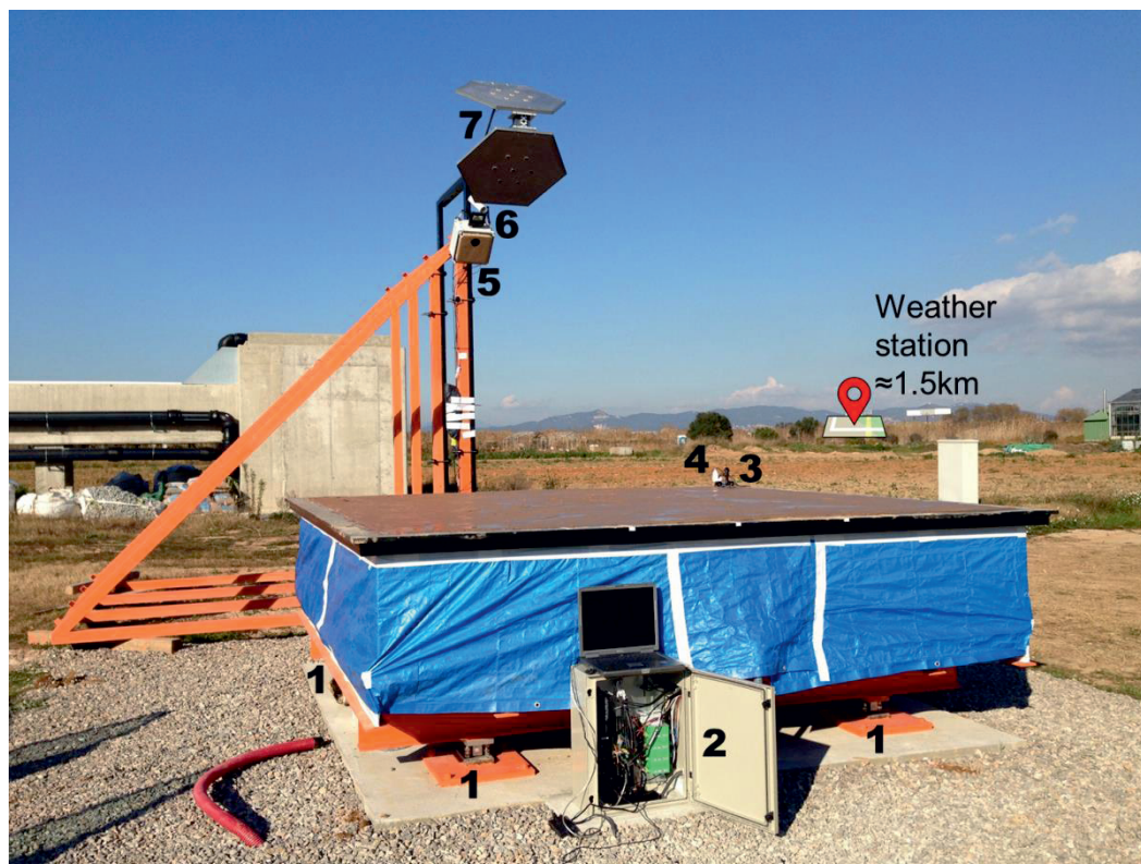
Figure 1. Overview of the field test. 1. Load cells; 2. Data recording system; 3. Anemometer; 4. VP-3 (Relative humidity, air temperature and vapour pressure sensors); 5. Digital camera; 6. IR-120 (infra-red remote temperature sensor); 7. RSLab reflectometer.
