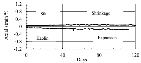
Figure 8. Change of axial strain with time for silt and kaolin.
