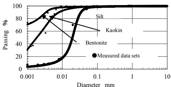
Figure 1. Grain size distribution for materials used in this test.
