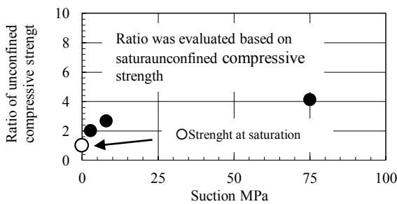
Figure 7. Influence of hydration effort on unconfined compressive strength.
