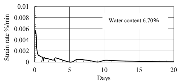
Figure 14 Strain rate in creep behaviour for bentonite with water content of 6.70 %.
