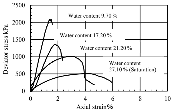
Figure 6. Stress-strain curve with various water contents for bentonite.
