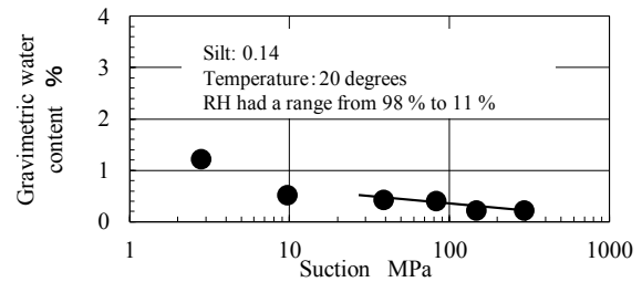
Figure 3. Soil-water characteristic curve for silt.
