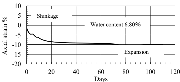
Figure 12. Creep behaviour for bentonite with water content of 6.80 %.
