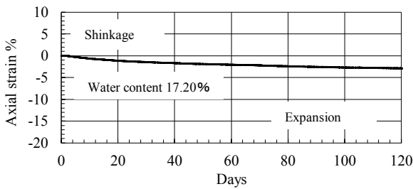
Figure 10. Creep behaviour for bentonite with water content of 17.20 %.
