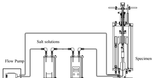
Figure 2. Modified creep test apparatus corresponding to RH control.
