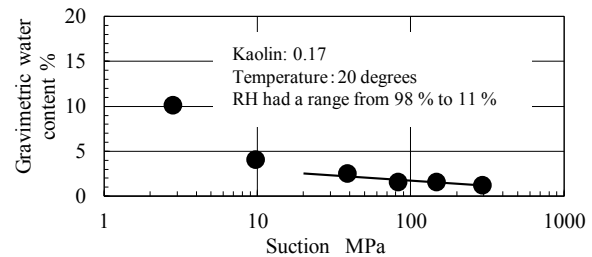
Figure 4. Soil-water characteristic curve for kaolin.
