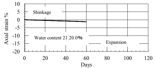
Figure 9. Creep behaviour for bentonite with water content of 21.20 %.
