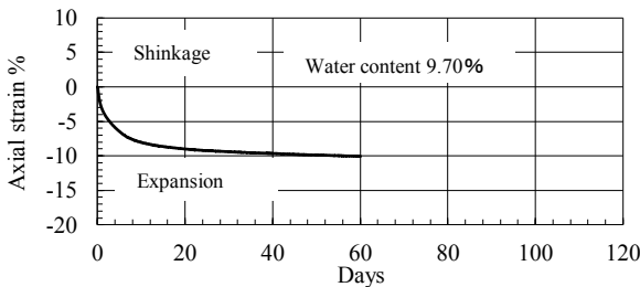
Figure 11. Creep behaviour for bentonite with water content of 9.70 %.
