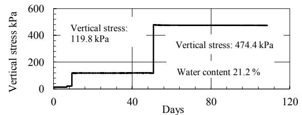
Figure 17. Different vertical stresses with elapsed time.
