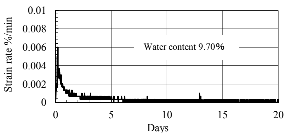
Figure 13. Strain rate in creep behaviour for bentonite with water content of 9.70 %.
