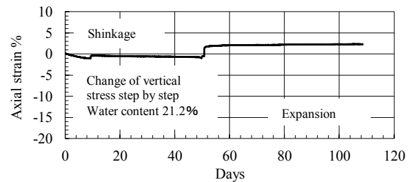
Figure 16. Creep behaviour for bentonite with water content of 21.20 % under different vertical stresses.
