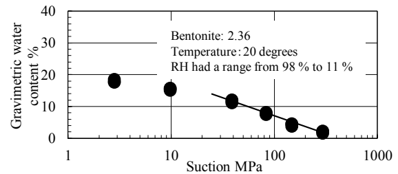
Figure 5. Soil-water characteristic curve for bentonite.
