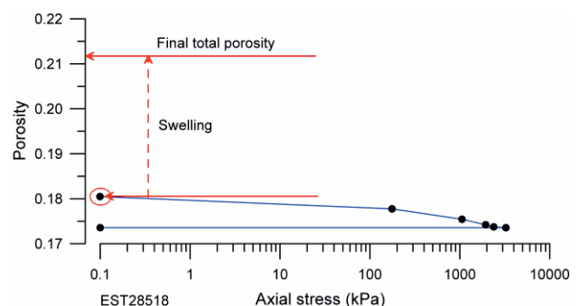
Figure 4. Unloading phase at constant water content
