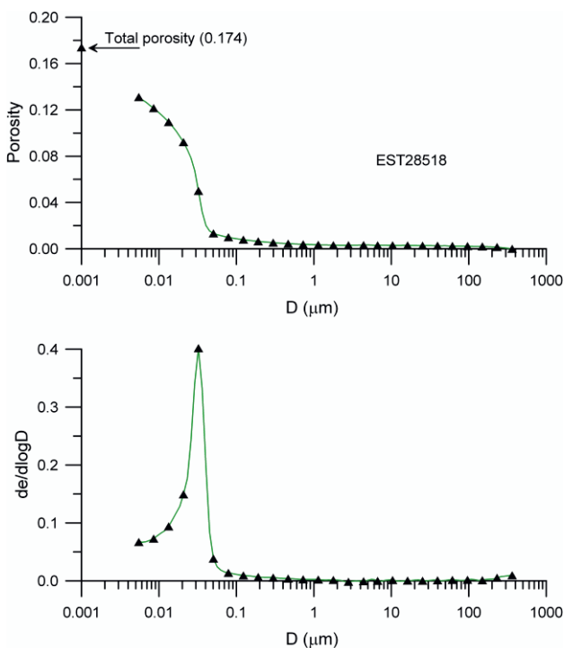
Figure 2. Pore size distribution curve initial state
