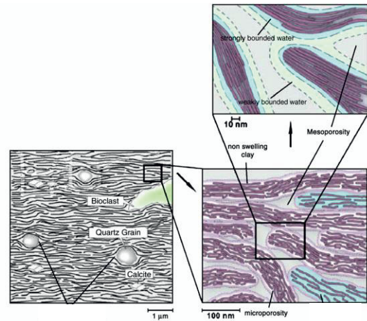
Figure 3. Microstructure model (after Yven et al., 14)
