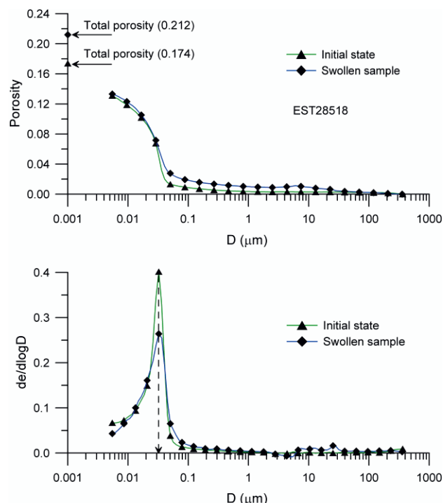
Figure 5. PSD curve of the swollen specimen
