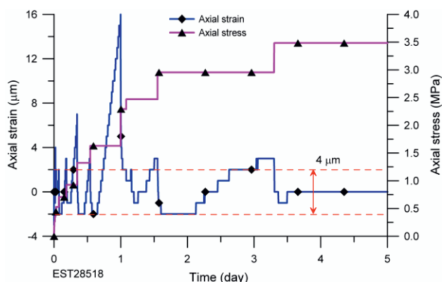
Figure 1. Resaturation with limited swelling
