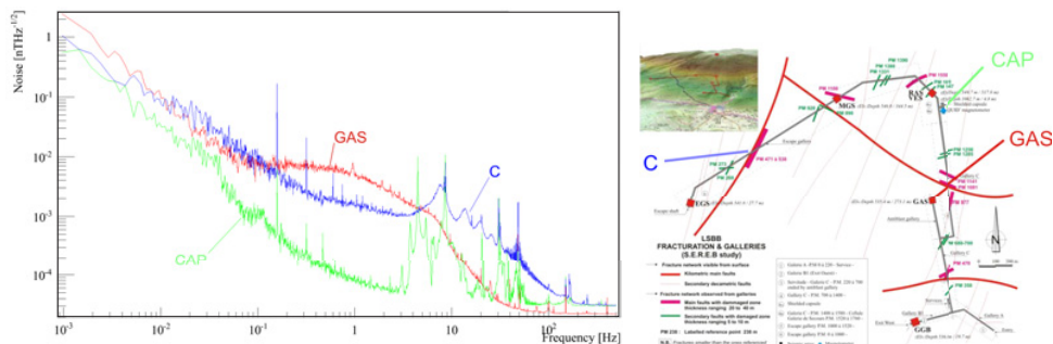
Figure 1. Left: frequency spectra of geomagnetic fluctuations recorded at different locations across the LSBB tunnel network: the shielded capsule (CAP), the GAS tunnel, and water flow point C. Right: a map of the LSBB laboratory showing the locations of the three measurement points.
