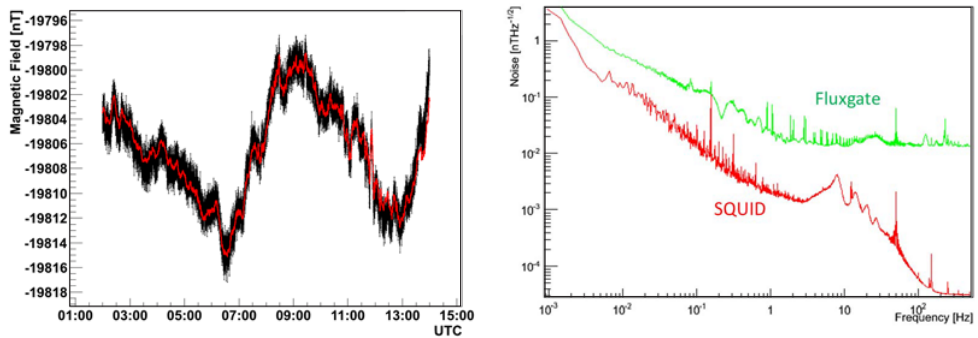
Figure 2. Left: magnetic signals recorded by the fluxgate (black line) and SQUID (red line) over a fourteen hour period. The 3-axis SQUID data has been transformed to fit this channel of the fluxgate to correct for difference in alignment of the two sensors. Right: frequency spectra of geomagnetic fluctuations recorded at point C using the SQUID (red) and fluxgate (green).
