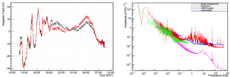
Figure 3. Left: magnetic signals recorded by fluxgate sensors at the Boulby Underground Laboratory (black line) and the INTERMAGNET data from the Eskdalemuir geomagnetic observatory, scaled to fit the Boulby data (red line). Right: frequency spectra of magnetic signals recorded at the Boulby Underground Laboratory (red), at LSBB using SQUIDs (pink) and fluxgates (blue). The data was not recorded synchronously. The spectrum of fluctuations recorded at Eskdalemuir is also shown (green).
