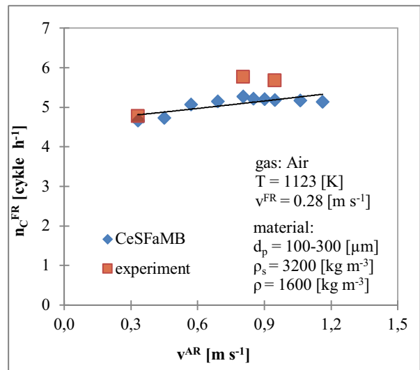
Fig. 19. The number of cycles in fuel reactor versus superficial gas velocity in the air reactor
