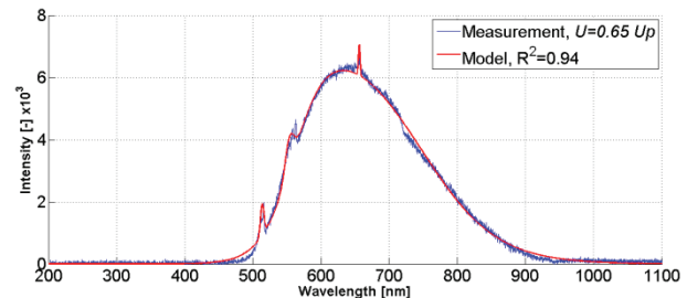
Fig. 6. Distribution of the spectrum of recorded optical radiation (blue color) and modeled (red) emitted by the ED generated in the point-point system in operated mineral oil with air bubbles for a relative supply voltage value of 0.65 U_b .
