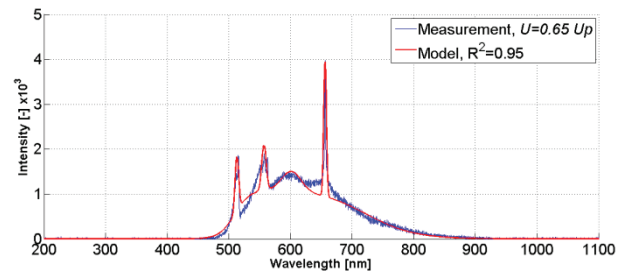
Fig. 5. Distribution of the spectrum of recorded optical radiation (blue color) and modeled (red) emitted by the ED generated in the point-plate system in operated mineral oil for a relative supply voltage value of 0.65 U_b .
