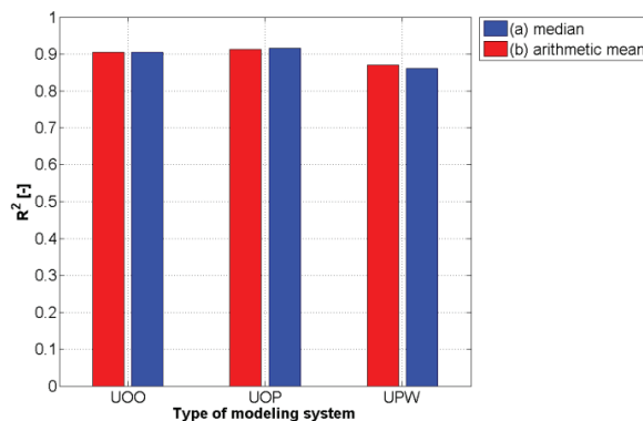
Fig. 11. Median (a) and arithmetic mean (b) of R^2 , calculated for ED generating systems: point-point (UOO), point-plate (UOP) and surface discharge system (UPW); generated in operated mineral oil.
