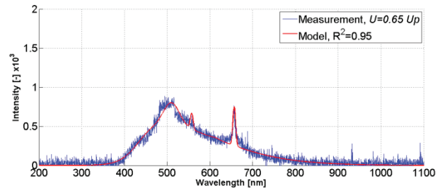
Fig. 4. Distribution of the spectrum of recorded optical radiation (blue color) and modeled (red) emitted by the ED generated in the point-plate system in pure mineral oil for a relative supply voltage value of 0.65 U_b .
