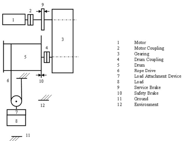
Fig. 1. Hoist Components.
