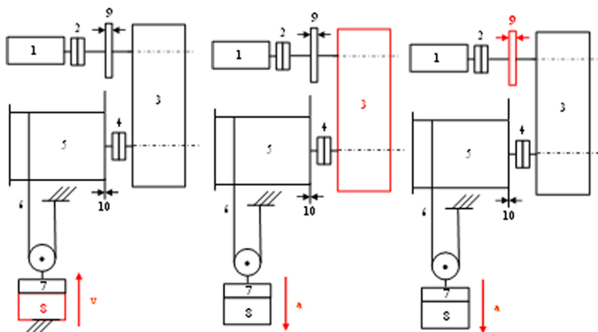
Fig. 4. Load cases overload, drivetrain failure, service brake failure.
