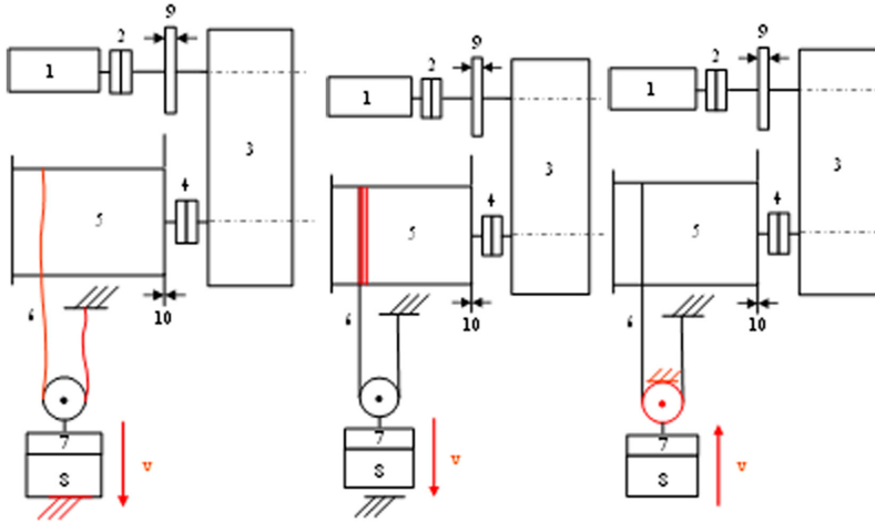
Fig. 3. Load cases slack rope, remaining rope windings, two blocking.
