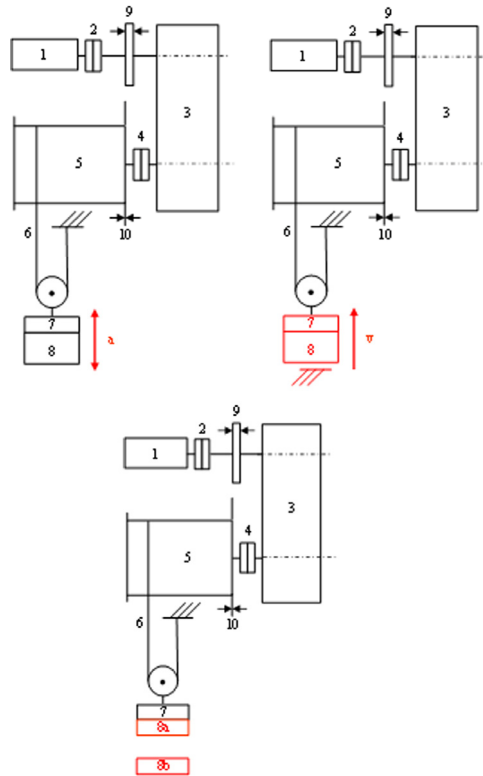
Fig. 2. Load cases acceleration/deceleration, Pick up of load and drop off of load.
