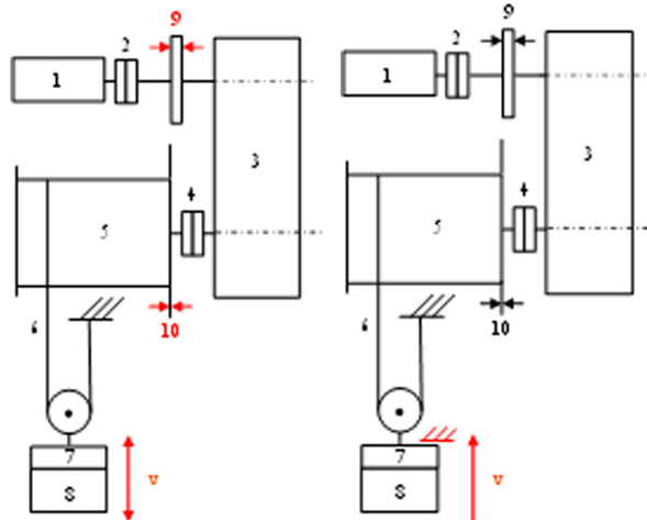
Fig. 5. Load cases emergency stop, snag.
