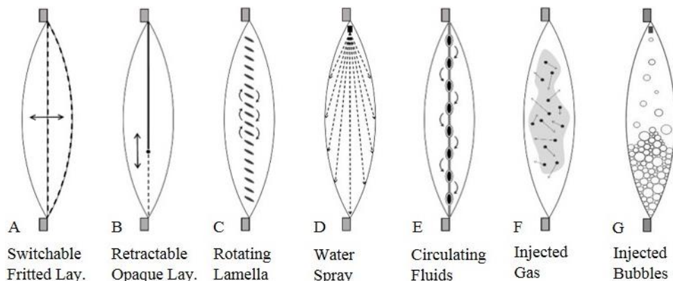
Fig. 3. Environmental control mechanisms for multilayer foil constructions.
