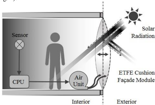
Fig. 2. Schematic diagram of a responsive building envelope incorporating a dynamic shading mechanism within a multilayer ETFE cushion.
