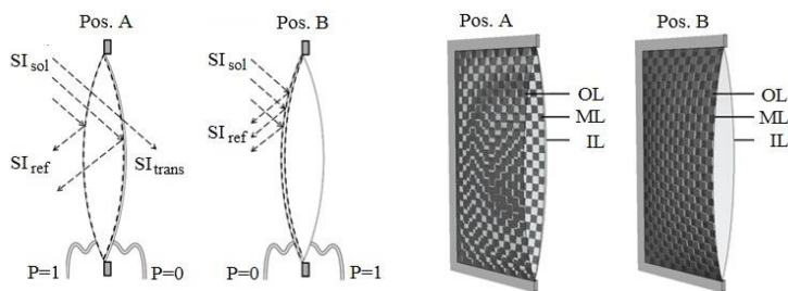
Fig. 4. Dynamic triple layer shading mechanism for pneumatic foil constructions, functional diagram and rendering of section in perspective view.
