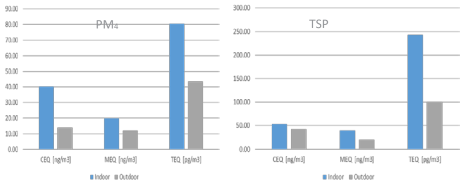
Fig. 3. Mean values of the risk indicators (CEQ, MEQ, TEQ) for PM 4 -bound and TSP-bound PAH in indoor (athletic hall) and outdoor (atmospheric) air.
