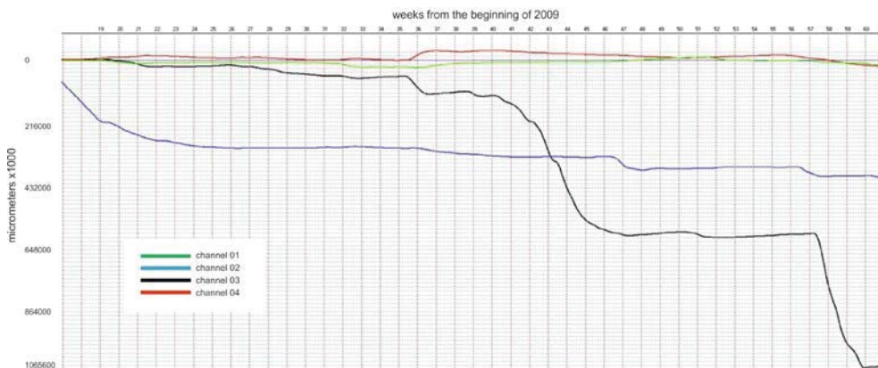
Fig. 3. Records from four measuring channels of water-tube tiltmeters from 2009.
