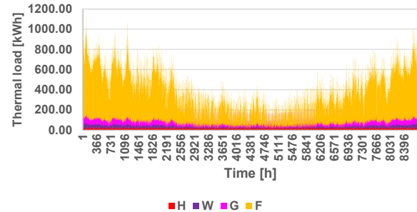
Fig. 9. The hourly components of the thermal load for the proposed situation
