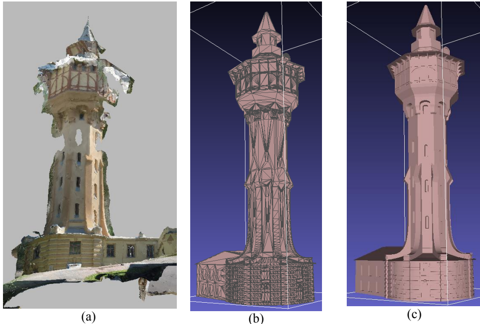
Fig. 2. (a) external colour model; (b) 3D mesh for BIM; (c) 3D BIM model.
