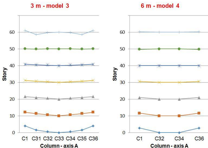
Fig. 10. Shear lag ratios distribution in rectangular buildings with different column spaces.
