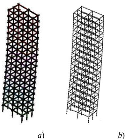
Fig.8. First mode of vibration: a) version 1; b) version 2
