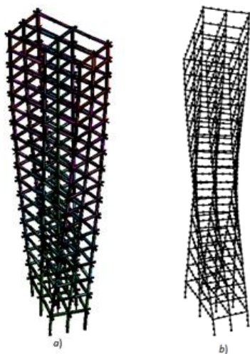
Fig.9. Third mode of vibration: a) version 1; b) version 2
