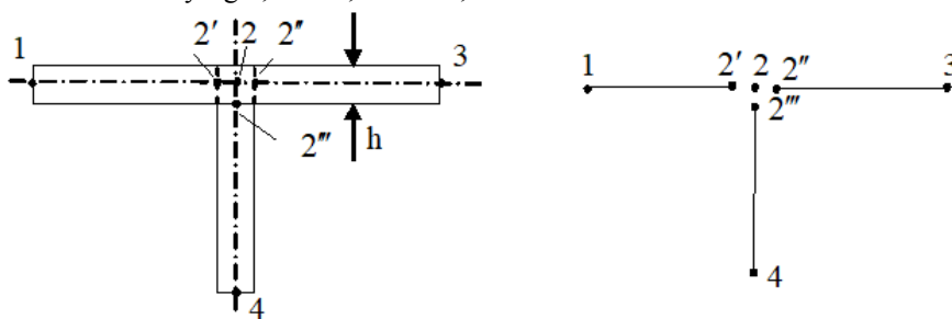
Fig.7. Connection of elements in the nodes of the design scheme with one-dimensional models of rods
