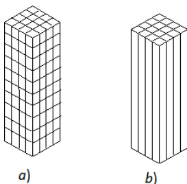
Fig.3. The superelement of the rod: a) partitioning of the rod on the volume finite elements; b) configuration of the grid after illumination of intermediate nodes
