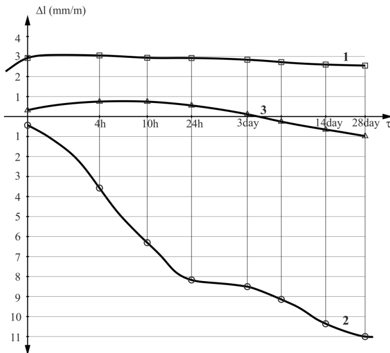
Fig. 1. Deformations of various binders (mm/m): 1 – gypsum; 2 – Portland cement; 3 – two-component binder
