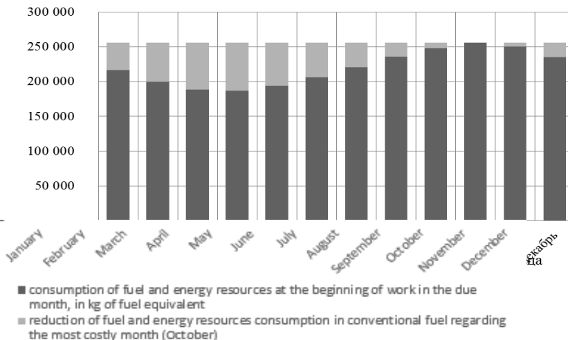
Fig. 2. Diagram of fuel and energy resources consumption changes depending on selection the month of beginning of the construction works
