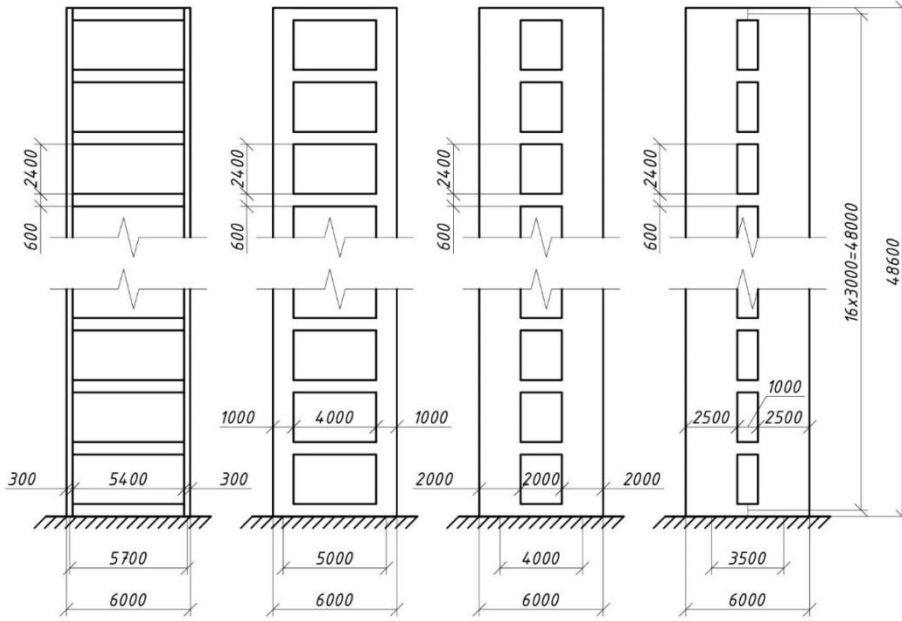
Fig. 3. A multi-story frame with its different proposals.
