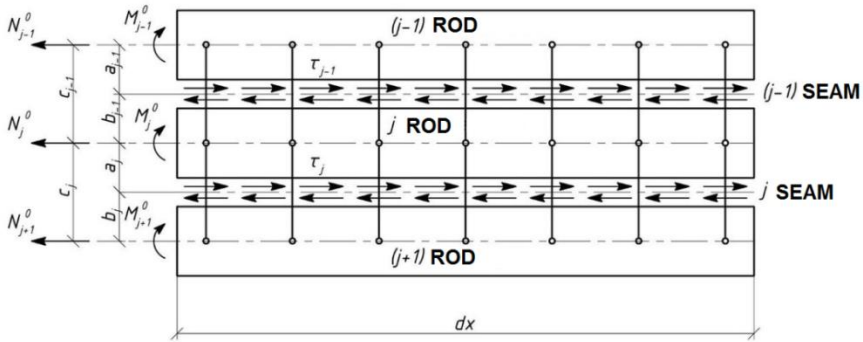
Fig. 1. Rigid linking in between individual beams.
