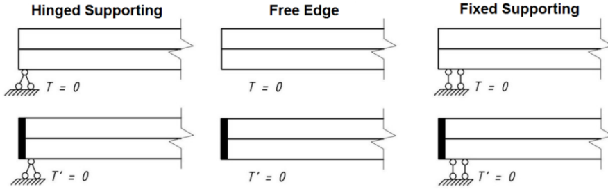
Fig. 2. Different boundary conditions.
