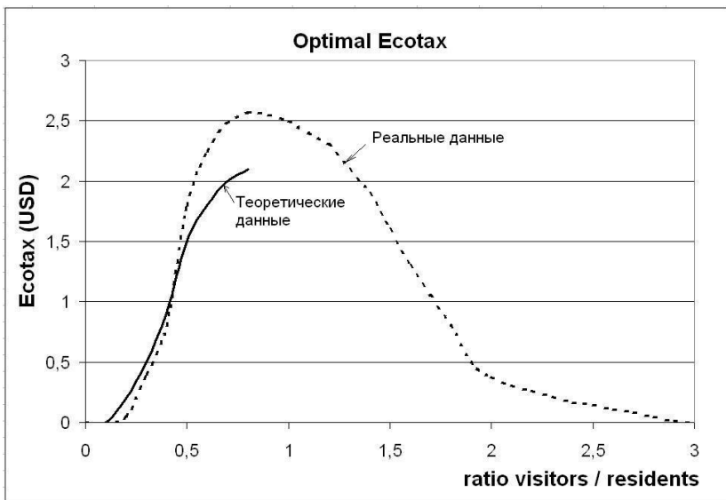
Fig. 3. Calculation of the optimal value Ecotax.
