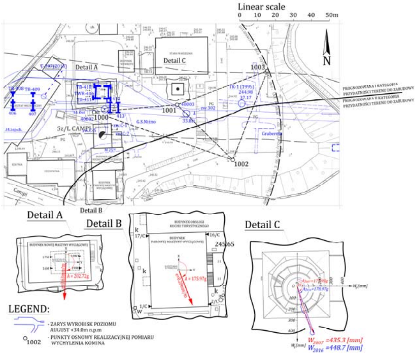
Fig. 2. Localization of the measurement stands on the background of situation details on the surface of mining excavations on Level August (the shallowest level connected with Shaft Camp1)
