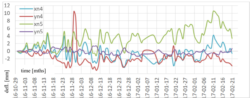
Fig. 6. Periodic deflection changes at the head (N4) and stem (N5) level, Daniłowicz shaft.
