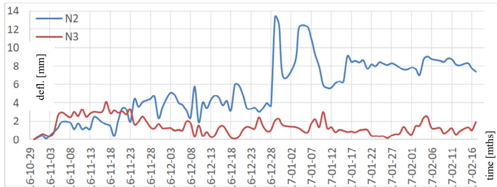
Fig. 5. Resultant deflection vectors at the head (N2) and stem (N3) level, St. Kinga shaft.
