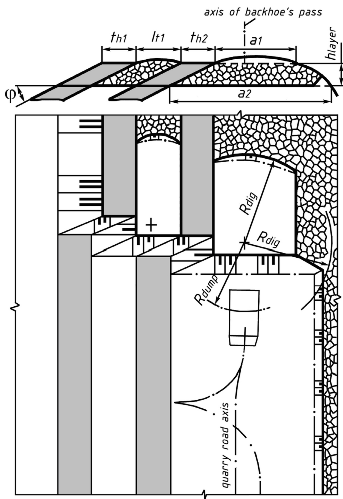
Fig. 1. Technological scheme of hydraulic backhoe use in the coal-bearing zone.
