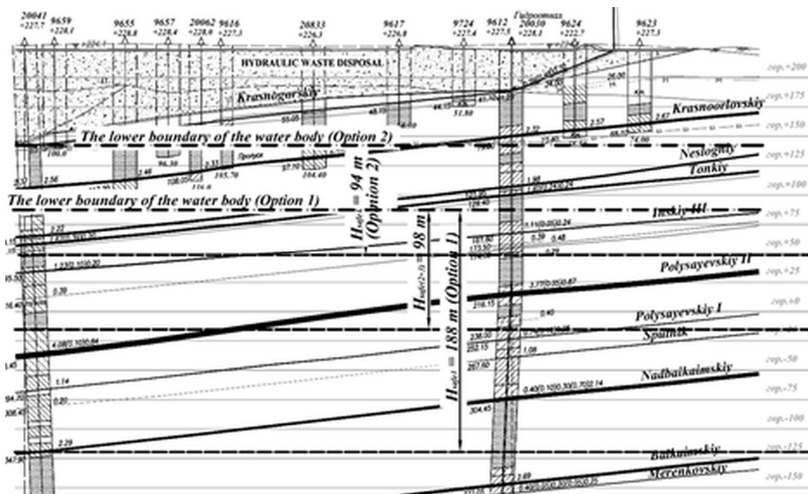
Fig. 1. Geological section along the exploration line with the design boundaries of the water body (in two options) plotted thereon, as well as safe mining depths for seam Polysaevskiy II ( H_{safe1} ) (in two options) and for joint mining of seams Nadbaikaimskiy and Baikaimskiy ( H_{safe(2+3)} ).
