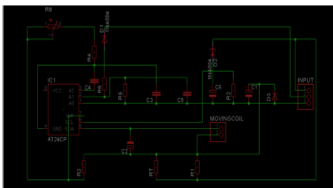
Fig. 2. Electronics circuit of analog tachometer
