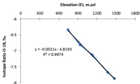
Fig. 4. Elevation versus isotope ratio of \delta^{18}\text{O} in rainwater sample
