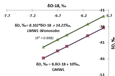
Fig. 3. LMWL Wonosobo and GMWL curve
