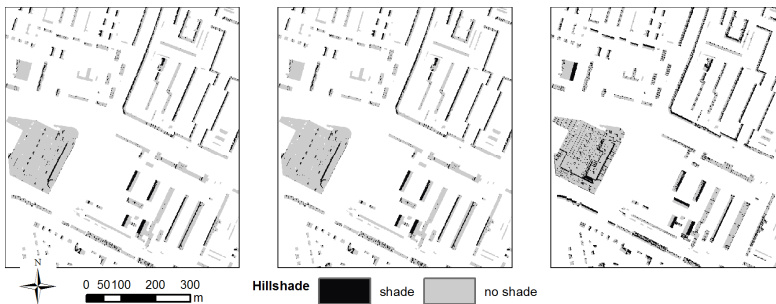
Fig. 7. Shading model of rooftops – March 21, 8 am; June 22, 12 pm and December 22, 3 pm.
