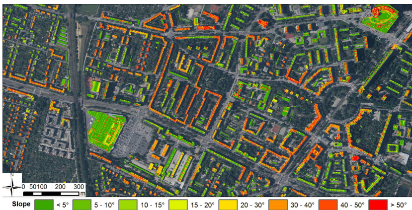
Fig. 5. Slope model of rooftops.
