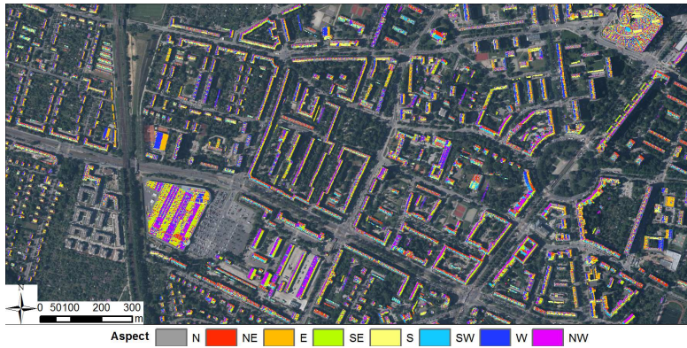
Fig. 6. Exposition model of rooftops.
