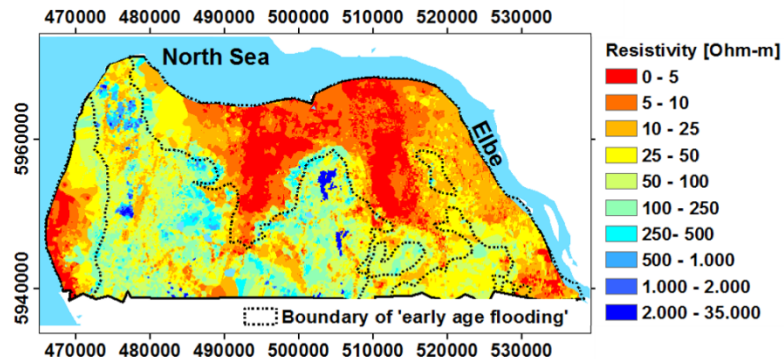
Figure 2. Resistivity distribution at 35 m to 40 m depth. Dotted line showed the boundary of ‘early age flooding’ (digitised after NIBIS® Kartenserver 2014b).
