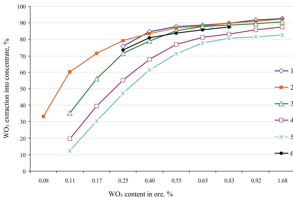
Fig. 1. The dependence of extraction of scheelite into saleable concentrate on the content of WO_3 in various types of ores and rocks: 1 – scheelite-quartz-sulphide ore; 2 – quartz metasomatites; 3 – biotite hornfels; 4 – skarns; 5 – skarnified hornfels; 6 – feed of Primorskaia ore-processing plant
