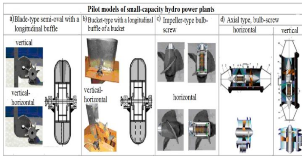
Fig. 2. Hydro turbine design approved for pilot-scale tests
