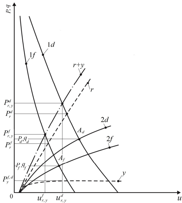
Fig. 2. The scheme of the loading, formed on the rigid ( r ) and yielding ( y ) components of the general fastening system in the mine working: 1 f and 1 d – deformation-strength characteristics of the weakening massif near the mine working contour in favourable ( f ) and difficult ( d ) mining and geological conditions; 2 f and 2 d – deformation-strength characteristics of natural equilibrium dome rocks; – – – deformation-strength characteristics of the rigid ( r ) and yielding ( y ) components of the fastening system; – · – general deformation-strength characteristics of the fastening system.
