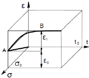
Fig. 3. Rheological model of gas hydrate compression at constant loading ( \sigma_i^* = \text{const} ).
