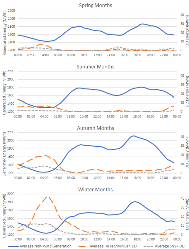
Fig. 2. Daily seasonal average of HighFreq/MinGen and SNSP against non-wind generation.
