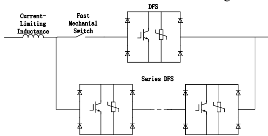
Fig.1 New Type Hybrid DC Breaker Topology
