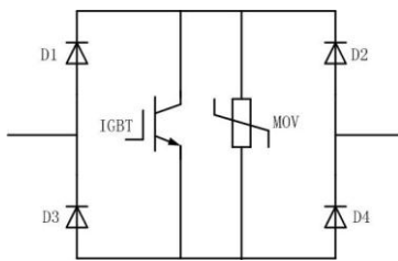
Fig.2 Diode Full-bridge Submodule Topology
