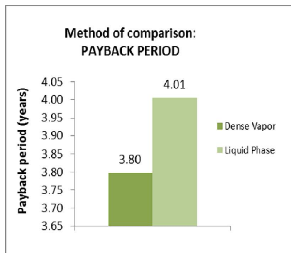
Figure 1. Comparison of PBP of the CO 2 phase schemes
