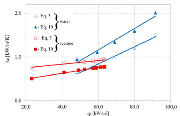
Fig. 5. Overall heat transfer coefficient vs. evaporator heat flux.
