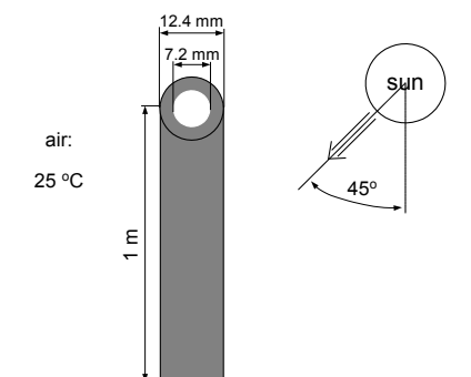
Fig. 2. An arrangement of the analyzed power cable.
