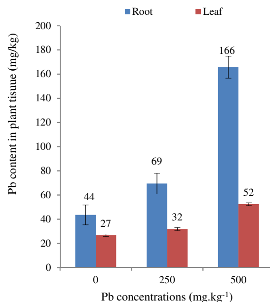
Fig 2. Lead accumulation within the plant tissues
