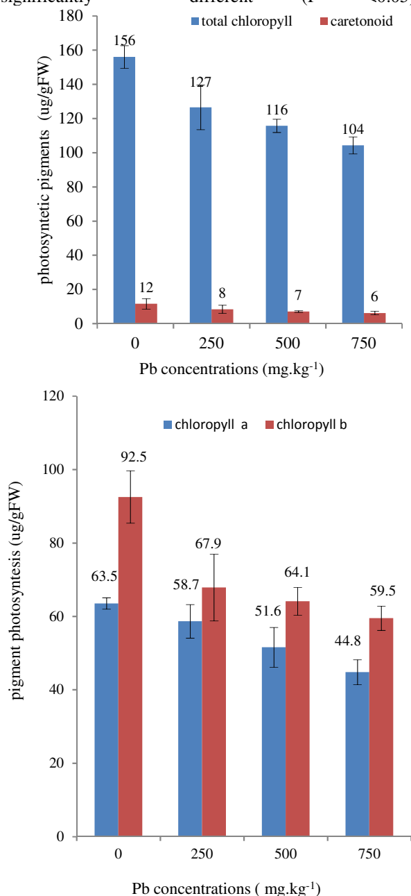
Fig.1. Effect of lead on photosynthetic pigment
