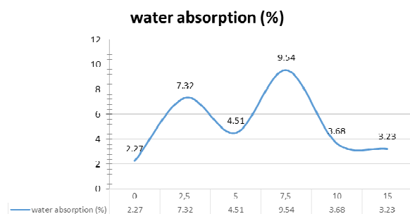
Figure 3. Water permeation average as paint sludge addition function.
