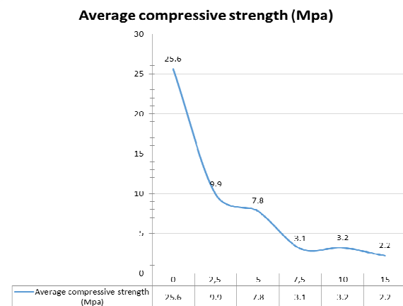
Figure 2. Compressive strength as paint sludge addition
