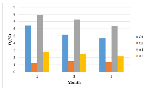
Fig. 5. Level of O 2 during experiment
