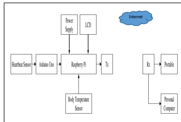
Figure 2. Hardware block diagram
