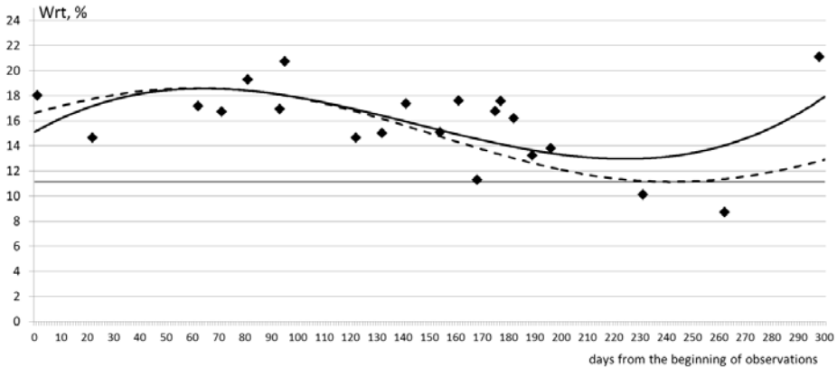
Fig.5 Change in the mass fraction of total moisture in the ash sampled basis of ordinary coal from the Jabariki-Khai coal field at the expense depot of the Deputatski Heat and Power Plant.
