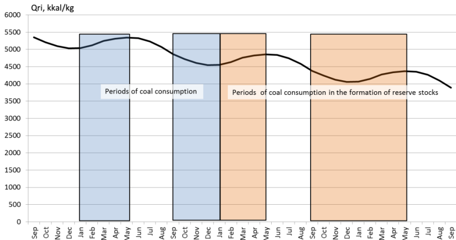
Fig.6 An example of modeling the dynamics of net calorific value changes of ordinary coal with existing transportation and storage technologies
