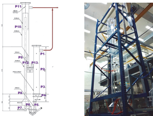
Fig. 5. The cold model of DFB gasification system: (a) Sketch of the cold model and the location of the pressure transmitters (P1~P13), and (b) the photo of the test apparatus.
