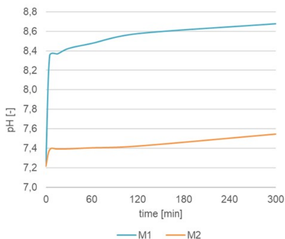
Fig. 5. Influence of adsorbing materials on pH of the effluent from HTW
