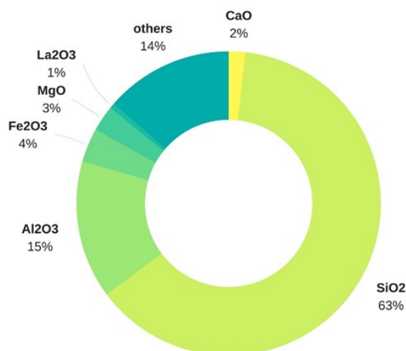
Fig. 2. Chemical composition of material M2
