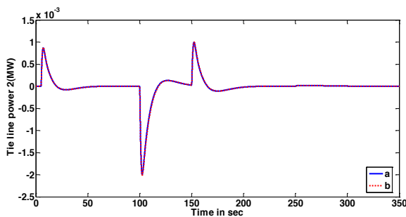
Fig. 9. Tie line power deviation for Area 2 and Area 3, solid line-a-nominal response, dotted line-b-perturbed response
