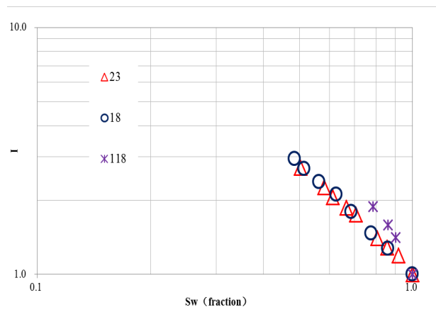
Fig 4. The relationship between m and K
