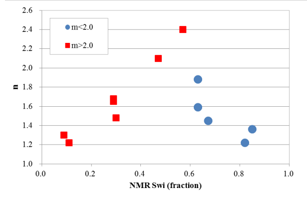
Fig 8. The relation between n and Sw_i
