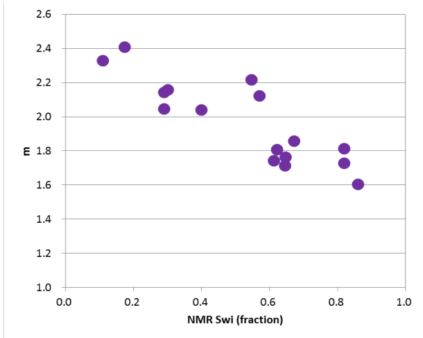
Fig 5. The relationship between m and Sw_i
