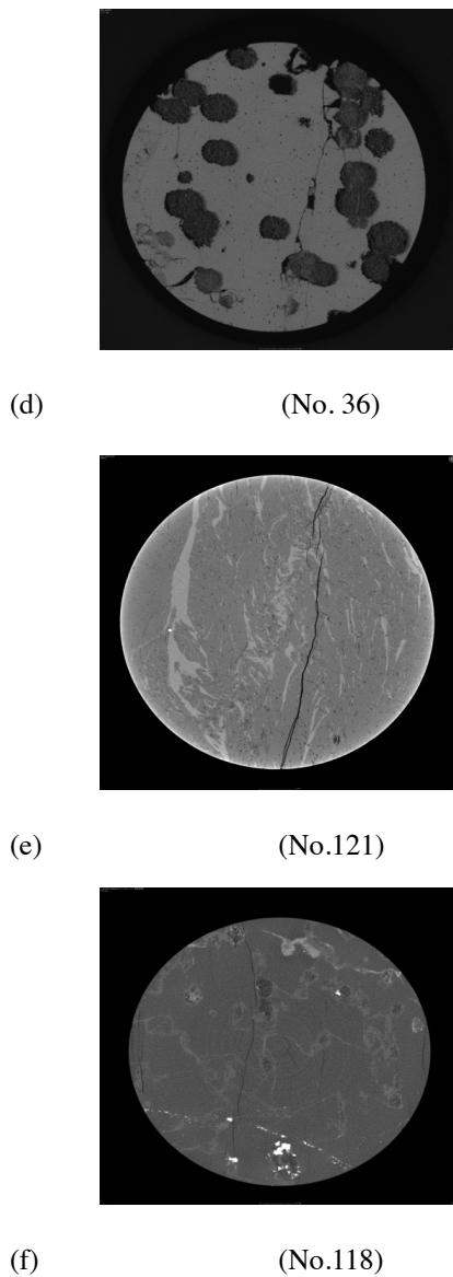
Fig.1 The Micro-CT images of the six typical carbonate samples
