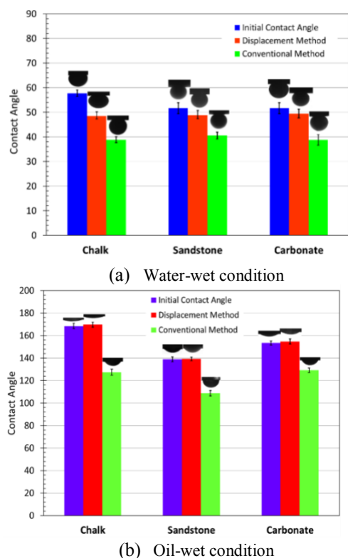
Fig. 7. Wettability alteration due to the presence of silica nanoparticles in complex systems
