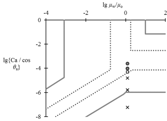
Fig. 2. Mobility ratio-Ca regime map. Marker shapes depict flow patterns observed in the displacement experiments: capillary fingering (cross), stable displacement (solid circle), and post-breakthrough sweep (squares). Superposed are regime boundaries for primary drainage proposed in the literature for uniformly wetting micromodels: a network of capillaries ([1], grey solid line) and a uniform cylinder array ([2], grey dotted). Adapted from [16].
