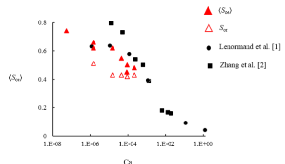
Fig. 7. \langle S_{oe} \rangle (solid triangles) and S_{or} estimated from history matching (open) as a function of Ca, plotted along measurements by Lenormand et al. [1] and Zhang et al. [2].
