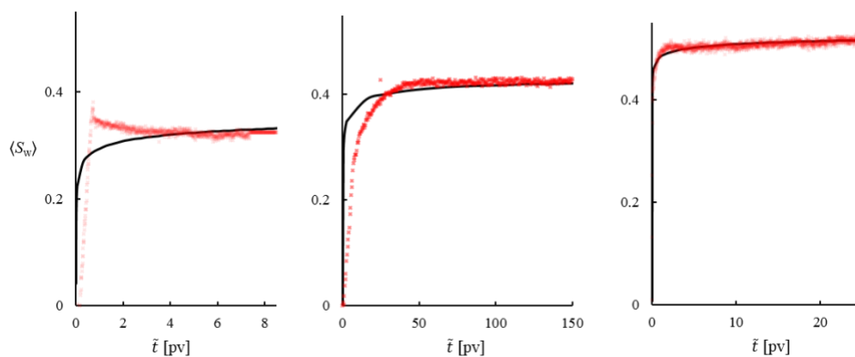
Fig. 4. Evolution of the remaining oil saturation as measured in the packed bed (red \times ) and simulated by history matching (solid line) for Ca = 1.5 \times 10^{-6} (left, M8), 4.6 \times 10^{-5} (middle), and 2.2 \times 10^{-4} (right). Where the solid line is not visible, it overlaps with the markers.
