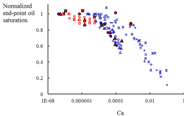
Fig. 5. End-point oil saturation normalized by its maximum value as a function of Ca under mixed-wet conditions (red) and uniformly water-wet conditions (blue) measured in Ketton (solid circle) and Indiana (solid square) limestones [24], in Whitestone and Edwards limestones by Tie & Morrow [25], in Berea sandstone by Chatzis & Morrow [23], and in five sandstones by Abrams [26] and \langle S_{oe} \rangle from the present study (red triangles). Expanded from Tanino et al. [24].
