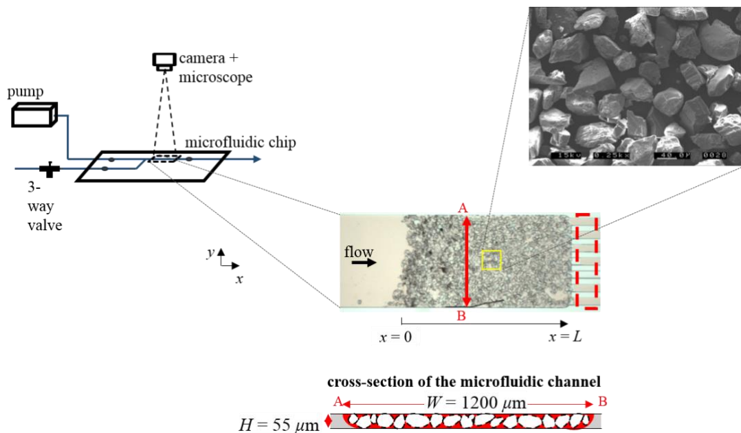
Fig. 1. The microfluidic setup (left) and scanning electron microscope (SEM) image of the grains (right). The dashed red rectangle demarcates the region downstream of the packed bed used to identify water breakthrough.
