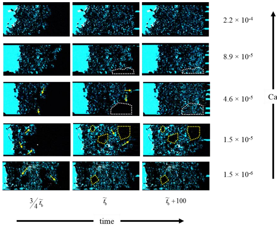
Fig. 3. Snapshots of the packed bed at \tilde{t} = 3\tilde{t}_b/4 , \tilde{t}_b , and \tilde{t}_b + 100 . An image at the onset of waterflood has been subtracted from each image and a 2 \times 2 median filter applied; bright pixels represent invading water. Imposed flow is from left to right. White dotted polygons demarcate regions invaded by water only after breakthrough. Yellow dotted polygons demarcate regions that remain unswept throughout the duration of the waterflood. Yellow arrows depict the direction of finger propagation as determined by visual inspection. From top to bottom: experiment M14, M21, M17, M5, and M7 (Table 2). Adapted from Ref. [16].
