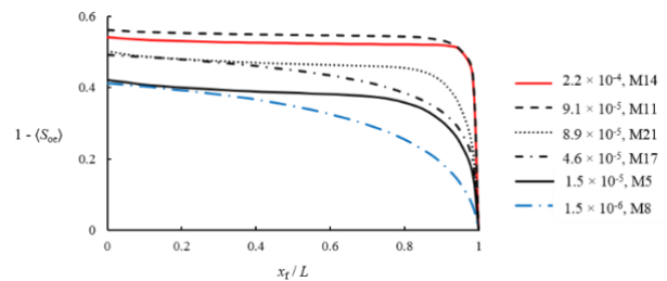
Fig. 6. End-point water saturation along the length of the packed bed at selected Ca: Ca = 1.5 \times 10^{-6} (blue dash-dotted), 1.5 \times 10^{-5} (black solid), 4.6 \times 10^{-5} (black dotted-dashed), 8.9 \times 10^{-5} (black dotted), 9.1 \times 10^{-5} (black dashed), 2.2 \times 10^{-4} (red solid).
