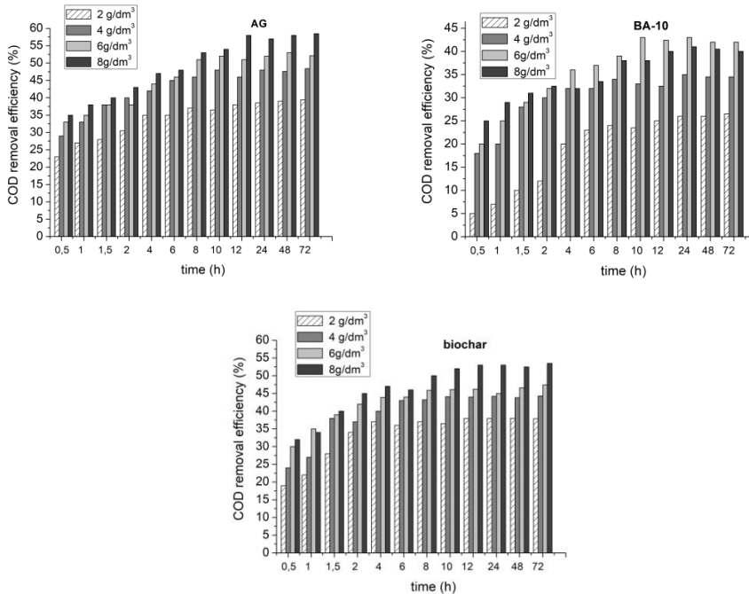
Fig. 1. Time determination of the sorption equilibrium for studied activated carbons and biochar.
